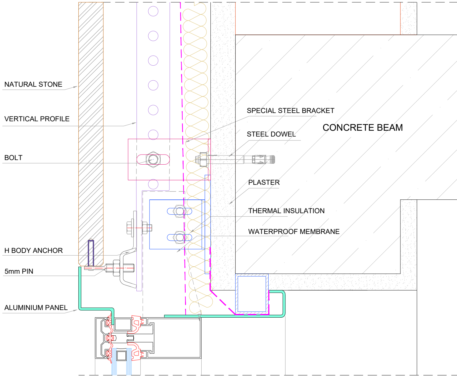
DETAIL B
