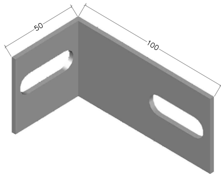
SPECIAL STEEL BRACKET
