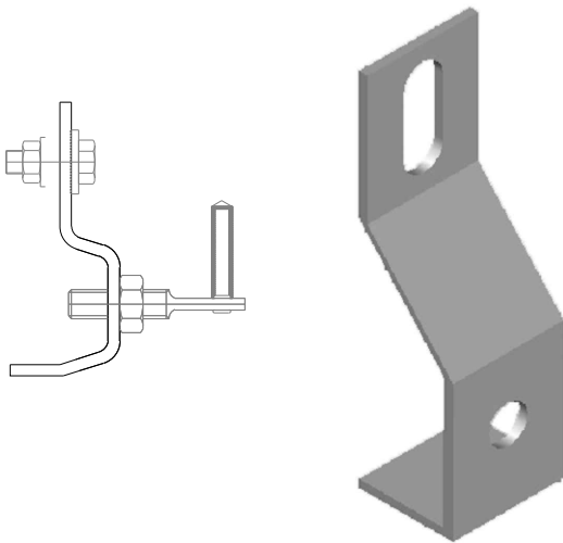
H BODY ANCHOR
